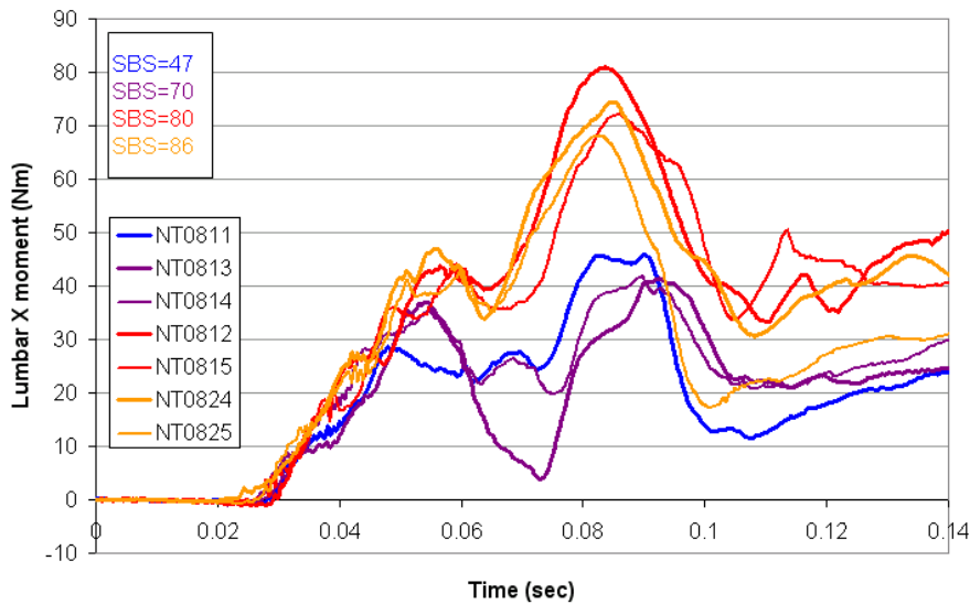
Figure 27. Lumbar X moment with variations in shoulder belt position.
