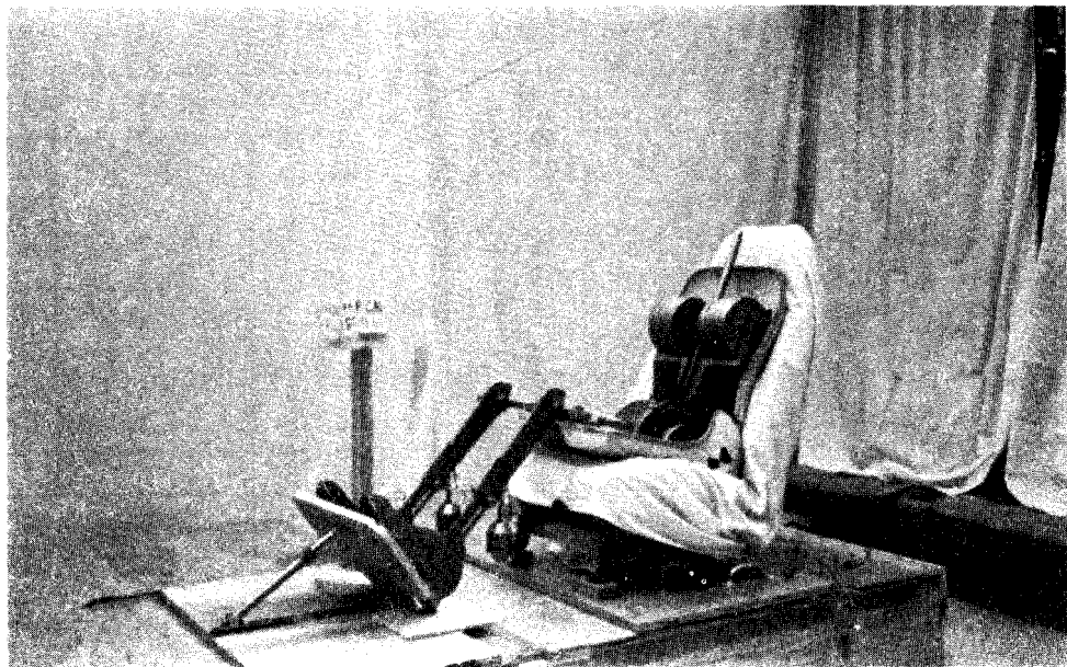
FIGURE 3-5. J826 H-point machine validation of vehicle seat bucks.
