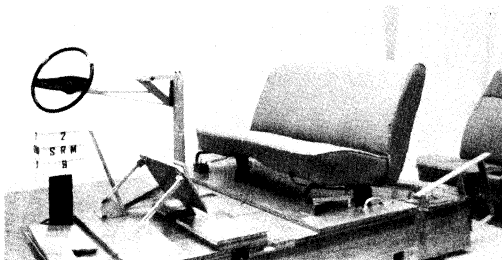
FIGURE 3-7. Phase II measurement buck with Malibu seat, toeboard, and steering wheel swung out of position.
