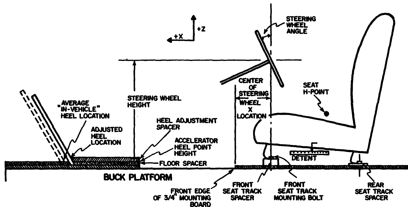
FIGURE C-1. Basic features of the vehicle seat buck.
