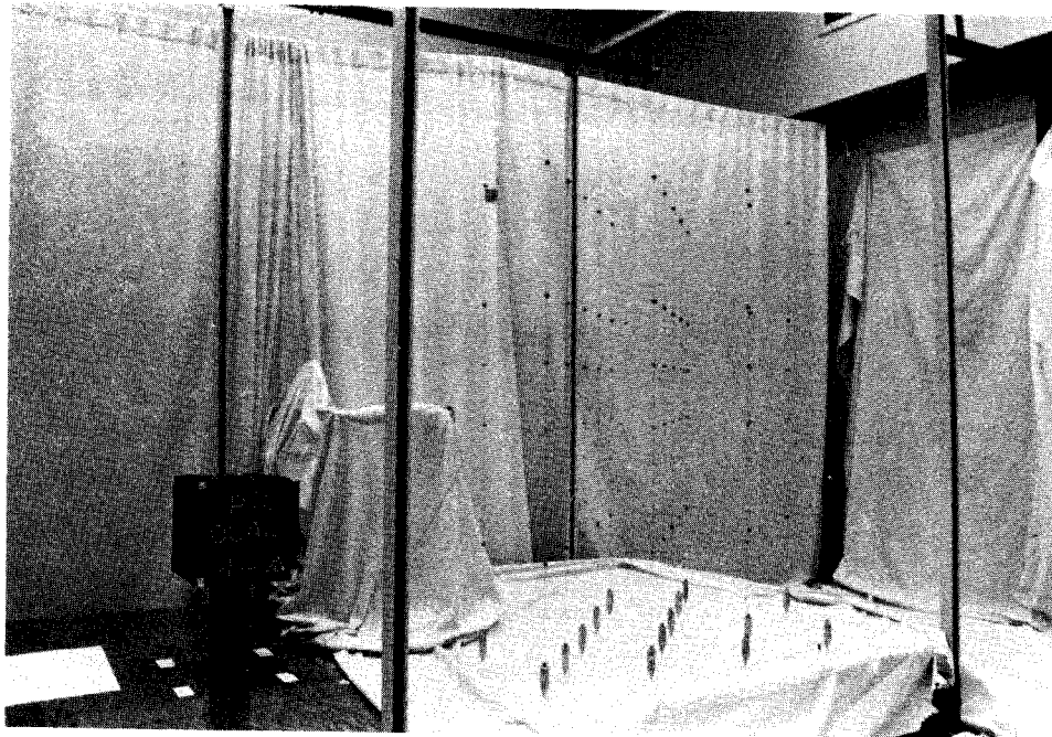
FIGURE 3-9. Target array for calibration of seven-camera stereophotogrammetry system.
