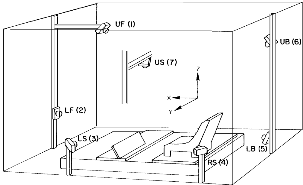
FIGURE 3-8. Schematic drawing of seven camera stereophotogrammetry system.
