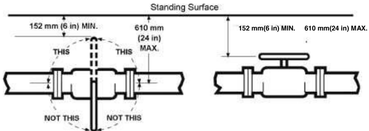
FIGURE 94. Mounting position for valve levers and handwheels below standing surface.
